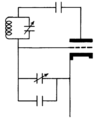
EQUIVALENT CIRCUIT
